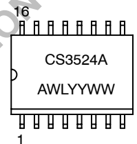
SO-16L DW SUFFIX CASE 751G
