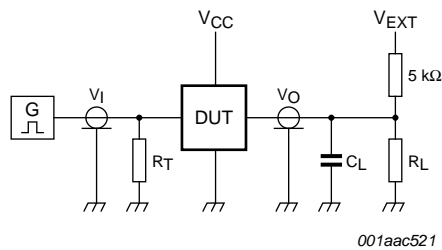
Test data is given in Table 10. Definitions for test circuit: RL = Load resistance. CL = Load capacitance including jig and probe capacitance. RT = Termination resistance should be equal to the output impedance Zo of the pulse generator. VEXT = External voltage for measuring switching times.
