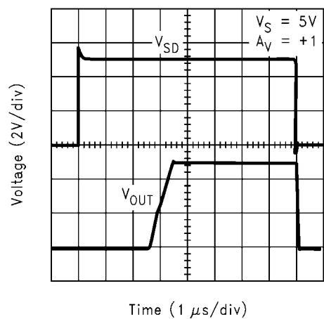
LMV711/LMV715 Turn On Characteristics
