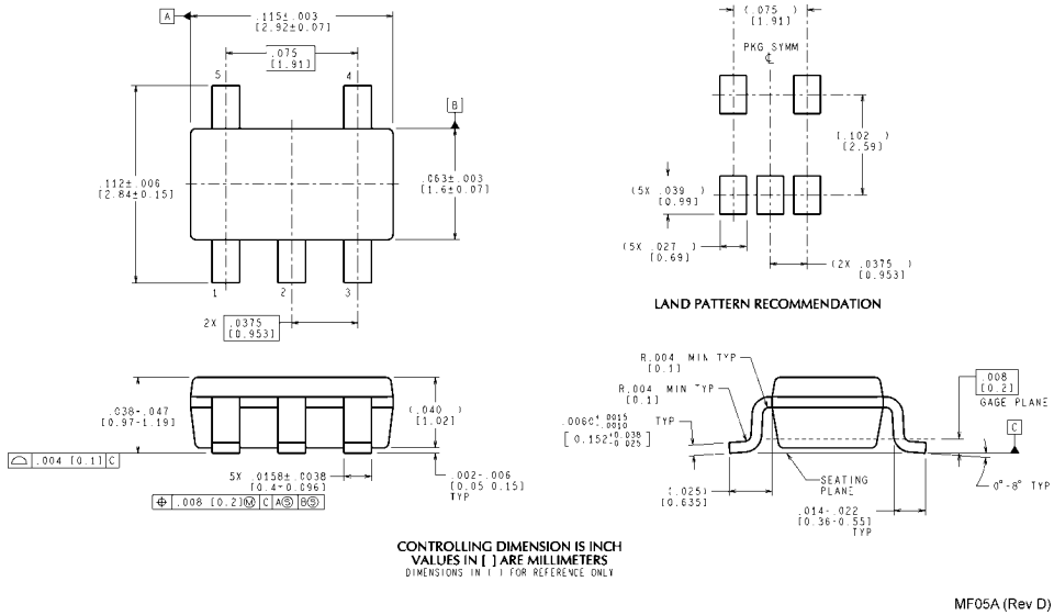
SOT23-5 NS Package Number MF05A
