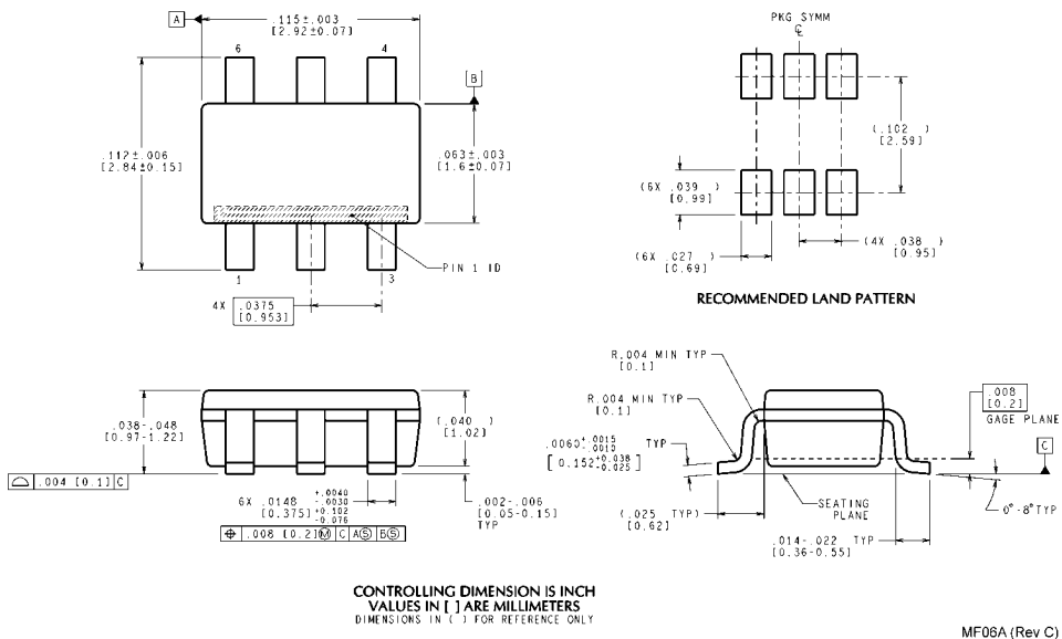
SOT23-6 NS Package Number MF06A
