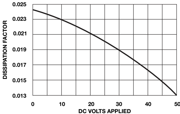
DISSIPATION FACTOR VS. VOLTAGE
