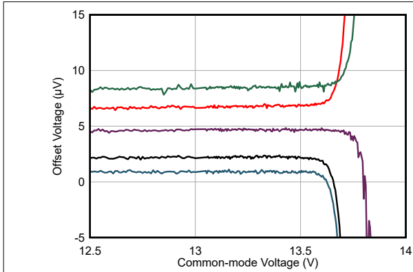
Figure 6-13. Offset Voltage vs V_{cm} at High Supply
