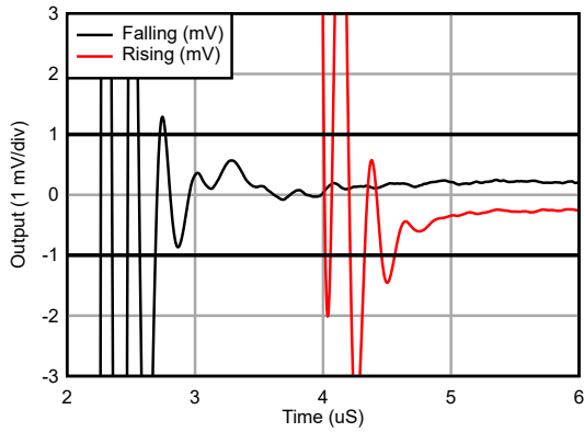
Figure 6-37. Settling Time
