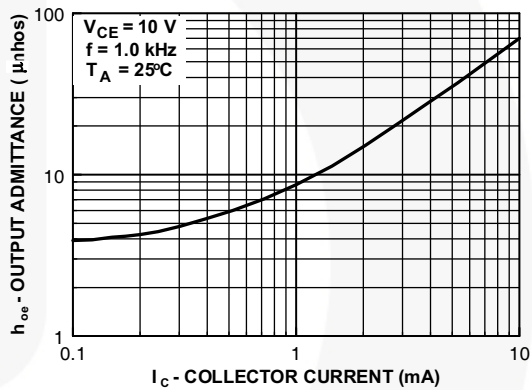
Figure 16. Output Admittance
