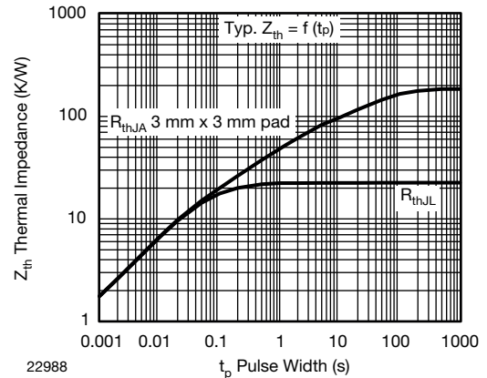
Fig. 6 - Typical Thermal Impedance vs. Time
