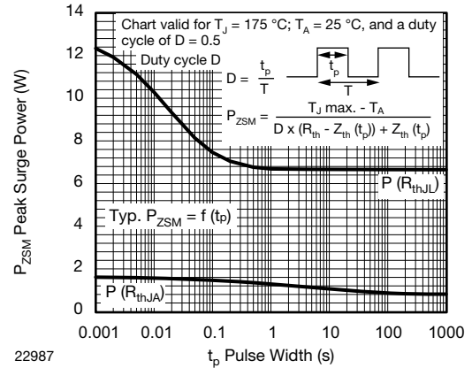
Fig. 5 - Typical Repetitive Peak Surge Power
