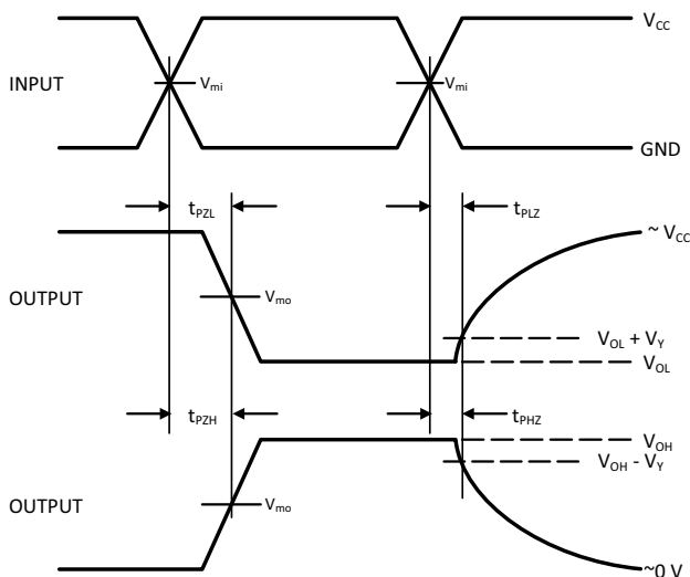
Figure 4. Switching Waveforms
