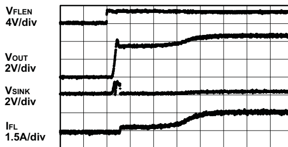
Time (40 \mu\text{s/div} )
