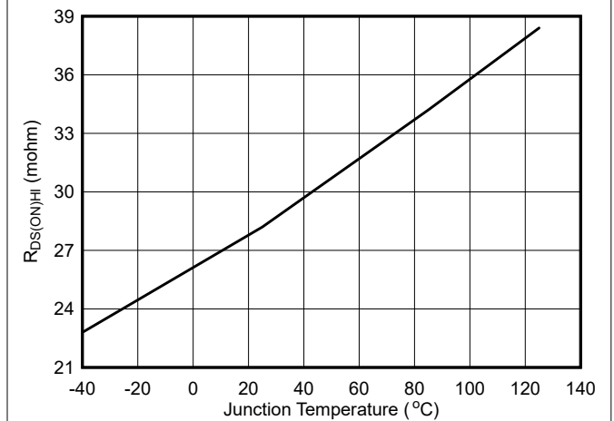
Figure 6-6. High-Side R_{DS(ON)}
