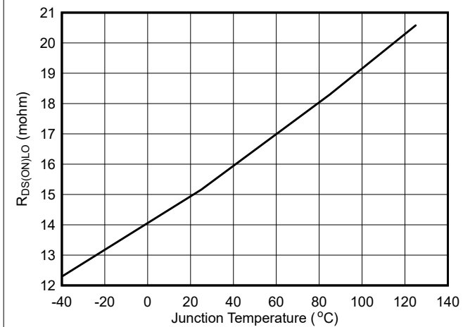
Figure 6-5. Low-Side R_{DS(ON)}
