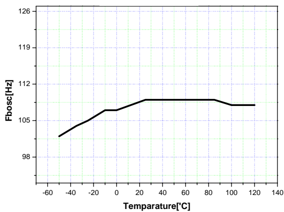
Figure 12. Operating Frequency
