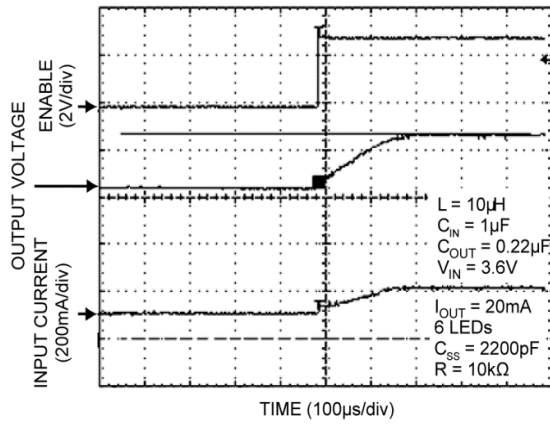
6-Series LED Circuit with External Soft-Start
