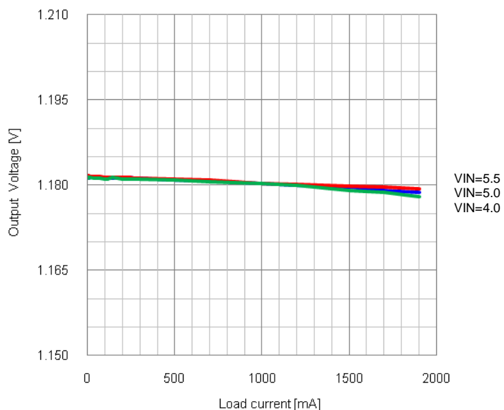
Figure 18. Load regulation PWM mode
