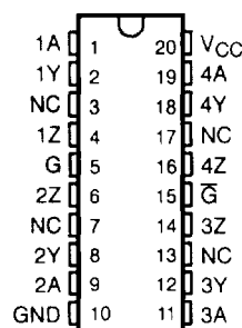
DW PACKAGE (TOP VIEW)
