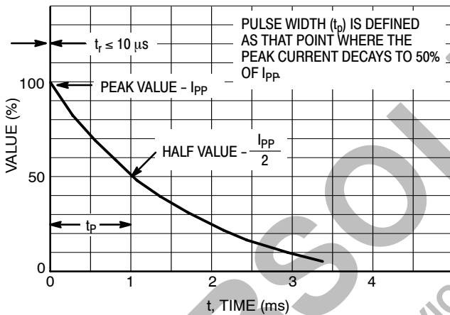
Figure 3. Pulse Waveform
