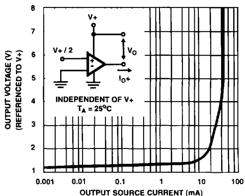
FIGURE 11. OUTPUT SOURCE CURRENT CHARACTERISTICS
