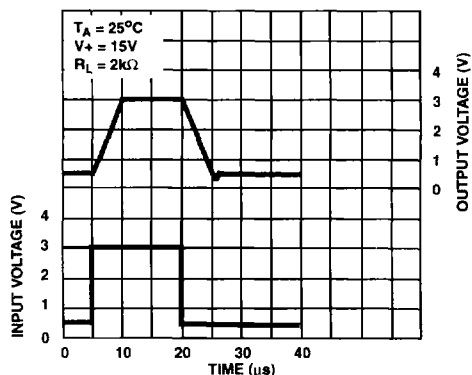
FIGURE 7. VOLTAGE FOLLOWER PULSE RESPONSE (LARGE SIGNAL)
