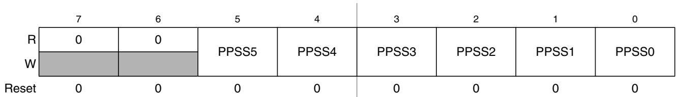
Figure 2-19. Port S Polarity Select Register (PPSS)
