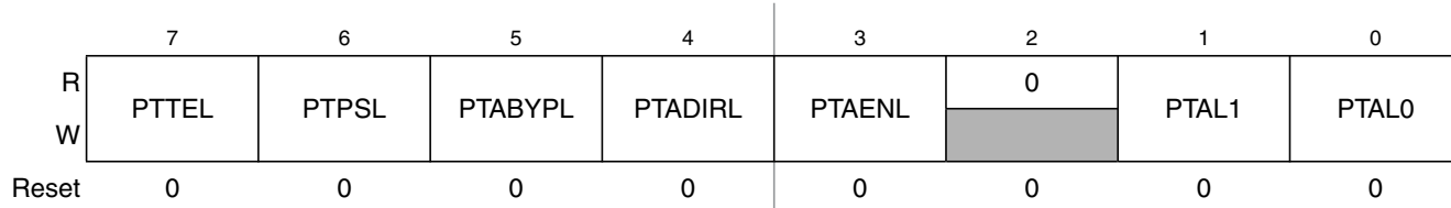
Figure 2-33. Port L Analog Access Register (PTAL)
