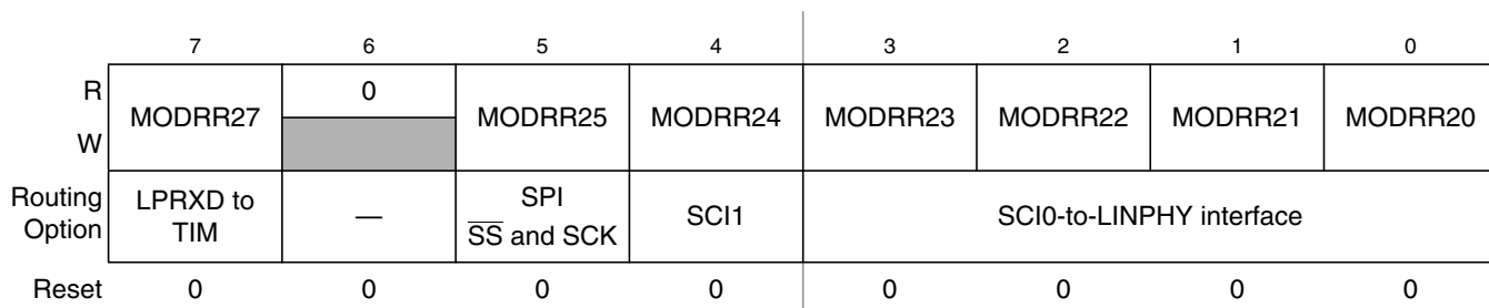
Figure 2-21. Module Routing Register 2 (MODRR2)
