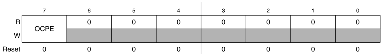
Figure 2-5. PIM Miscellaneous Register (PIMMISC)
