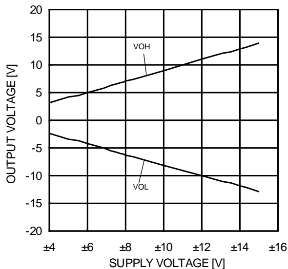
Figure 73. Maximum Output Voltage -Supply Voltage ( R_L=2k\Omega , T_A=25^{\circ}C )
