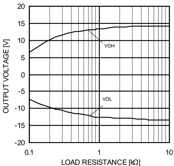
Figure 72. Maximum Output Voltage -Load Resistance ( V_{CC}/V_{EE}=+15V/-15V , T_A=25^{\circ}C )
