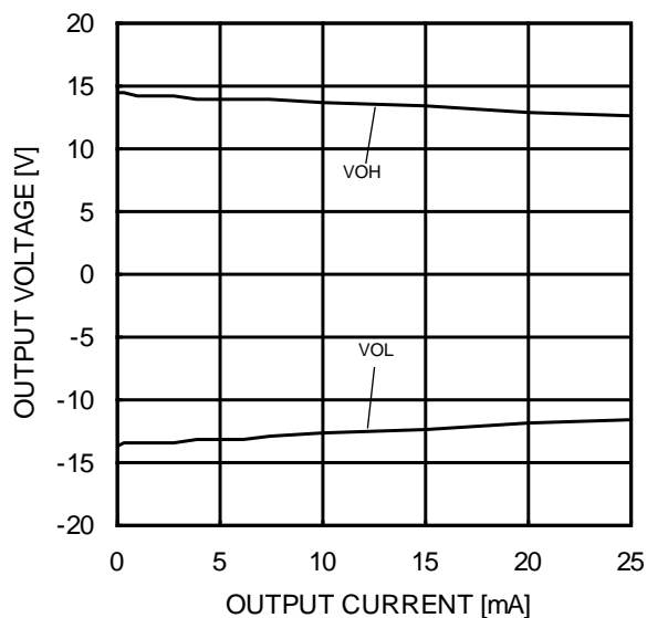
Figure 75. Maximum Output Voltage - Output Current ( V_{CC}/V_{EE}=+15V/-15V , T_A=25^{\circ}C )
