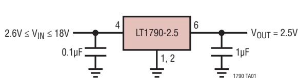
Positive Connection for LT1790-2.5
