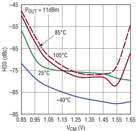
HD3 at 70MHz vs V_{CM} Over Temperature
