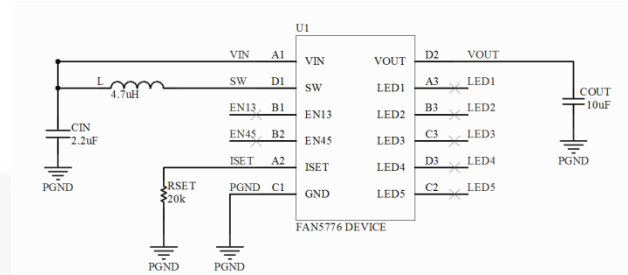
Figure 28. Schematic for Recommended Layout
