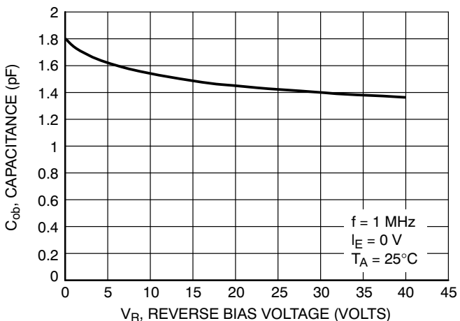
Figure 54. Output Capacitance
