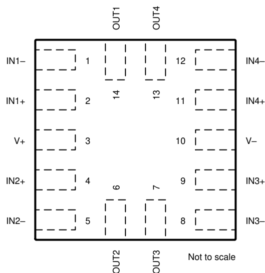
Not to scale Figure 6-11. OPA4310 RUC Package 14-Pin X2QFN (Top View)
