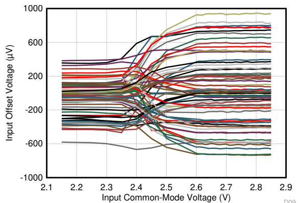
Figure 7-9. Offset Voltage vs Common-Mode
