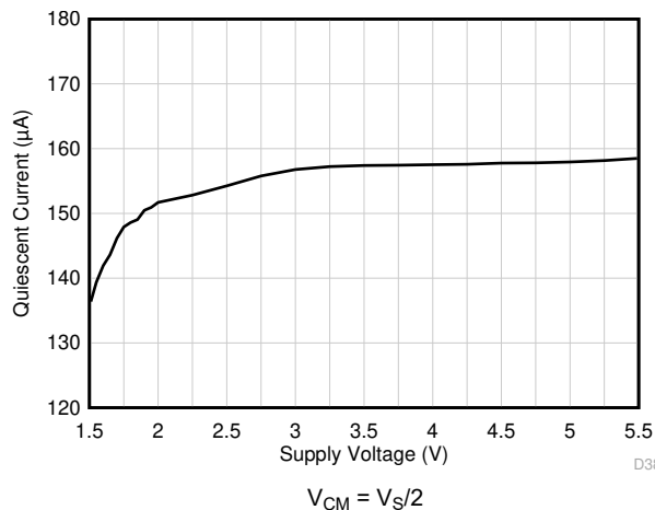
Figure 7-35. Quiescent Current vs Supply Voltage
