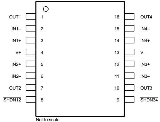
Figure 6-13. OPA4310S DYY Package 16-Pin SOT-23-THIN (Top View)
