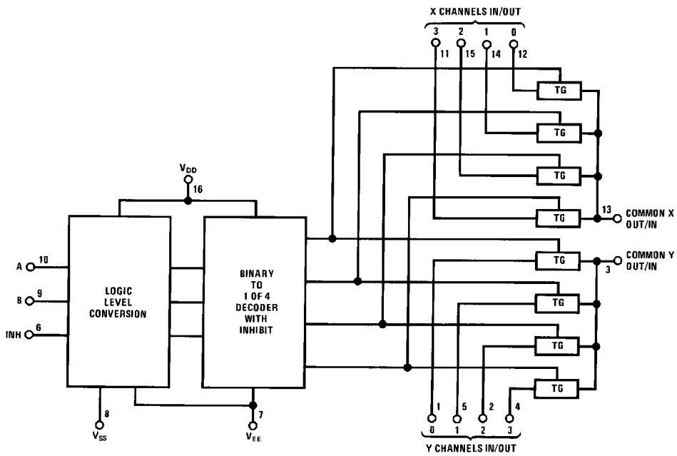
CD4052BM/CD4052BC
