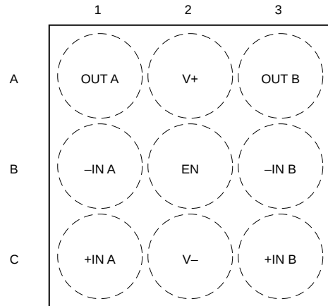
Figure 6-5. OPA2392 YBJ Package, 9-Pin DSBGA (Top View)
