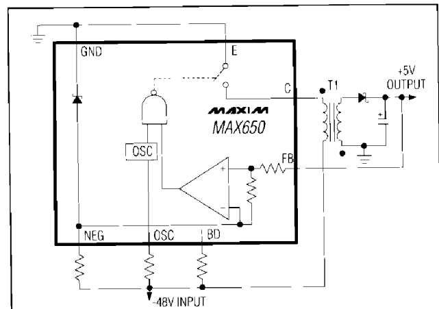
Figure 3. Typical Circuit
