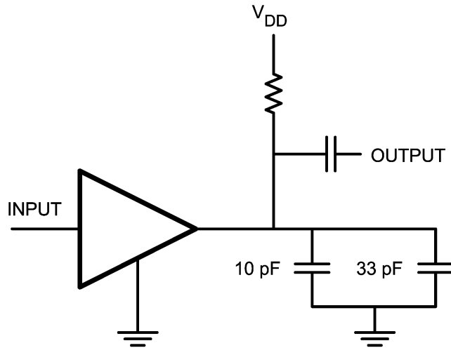
FIGURE 6. RF Noise Reduction
