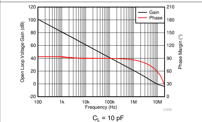
Figure 7-6. Open-Loop Gain and Phase vs Frequency
