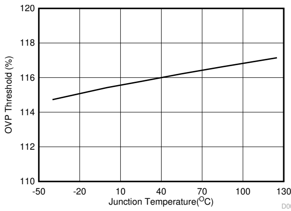
Figure 5-11. OVP Threshold vs Junction Temperature
