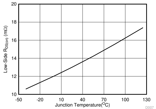
Figure 5-8. Low-Side R_{DS(on)} vs Junction Temperature
