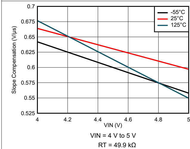
Figure 8-71. Slope Compensation Variation
