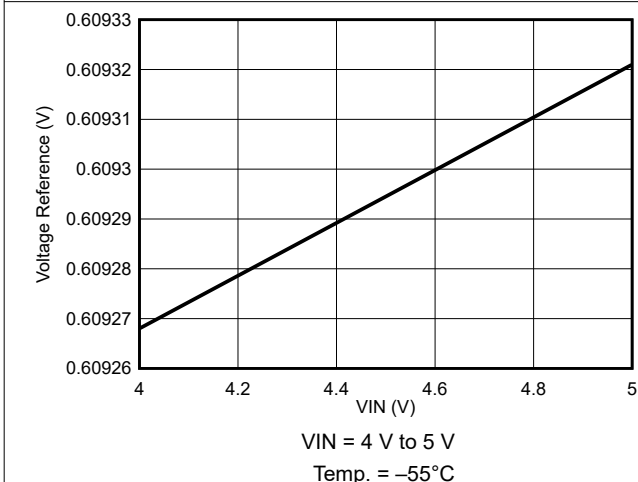
Figure 8-11. Voltage Reference Variation
