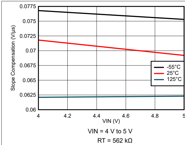
Figure 8-67. Slope Compensation Variation
