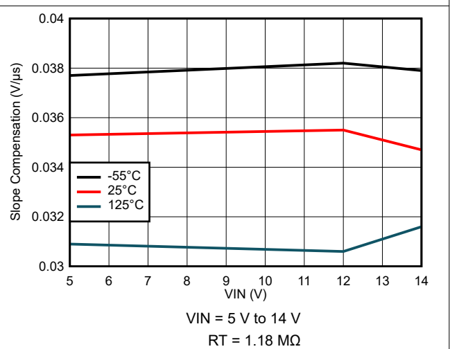
Figure 8-66. Slope Compensation Variation
