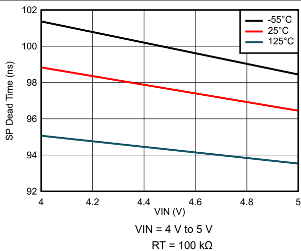
Figure 8-53. SP Dead Time Variation
