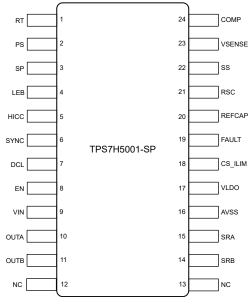
Figure 7-5. TPS7H5001-SP PW Package 24-Pin TSSOP (Top View)
