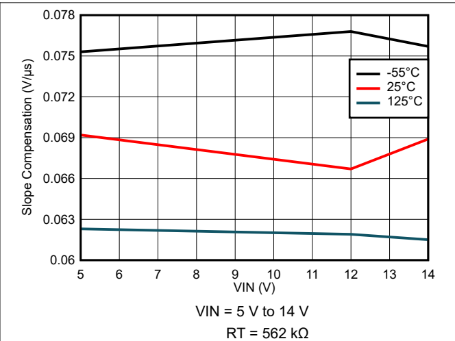
Figure 8-68. Slope Compensation Variation
