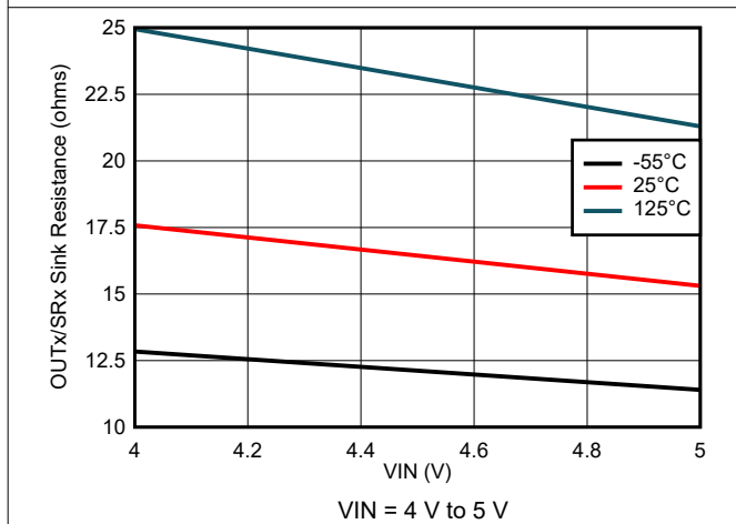
Figure 8-63. Output Sink Resistance Variation
