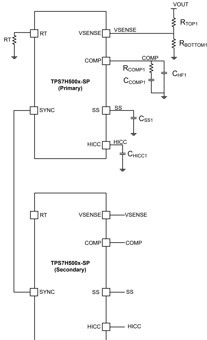
Figure 9-11. Primary-Secondary Mode Configuration for Parallel Operation
