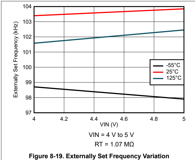
Figure 8-19. Externally Set Frequency Variation
