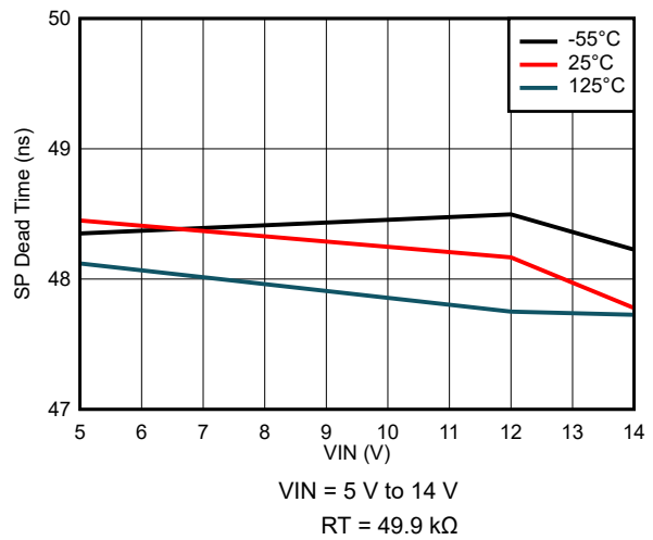
Figure 8-52. SP Dead Time Variation
