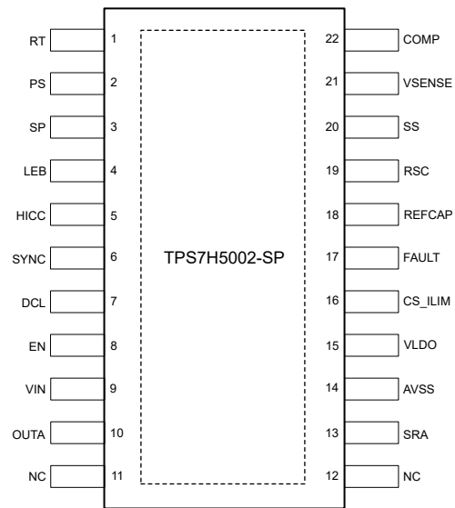
Figure 7-2. TPS7H5002-SP HFT Package 22-Pin CFP With Thermal Pad (Top View)
