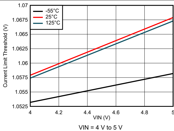
Figure 8-17. Current Limit Threshold Variation
