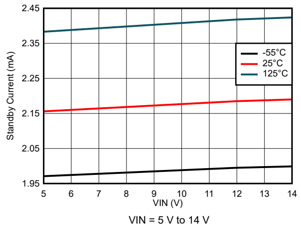
Figure 8-4. Standby Current Variation
