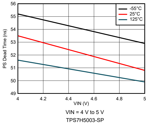
Figure 8-47. PS Dead Time Variation
