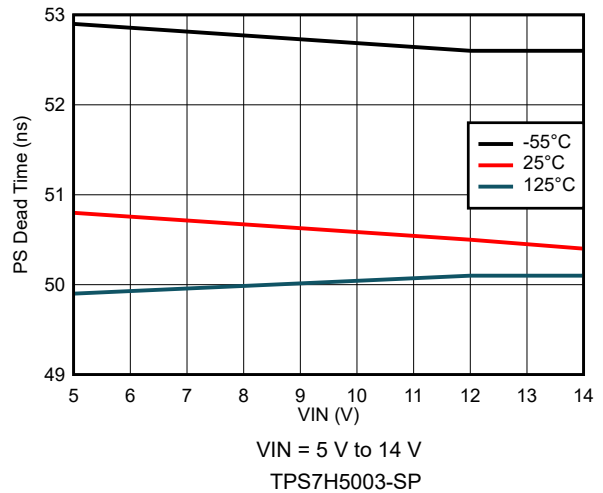
Figure 8-48. PS Dead Time Variation
