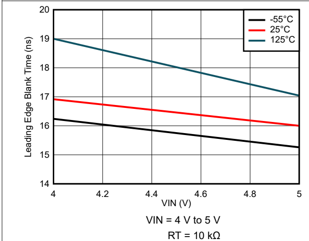
Figure 8-33. Leading Edge Blank Time Variation
