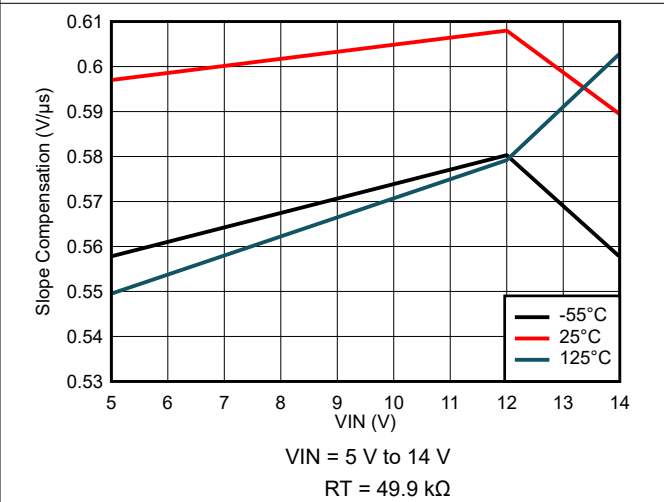
Figure 8-72. Slope Compensation Variation
