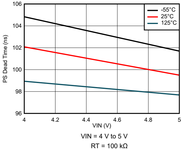
Figure 8-45. PS Dead Time Variation
