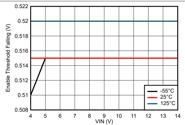
Figure 8-8. Enable Threshold Falling Variation
