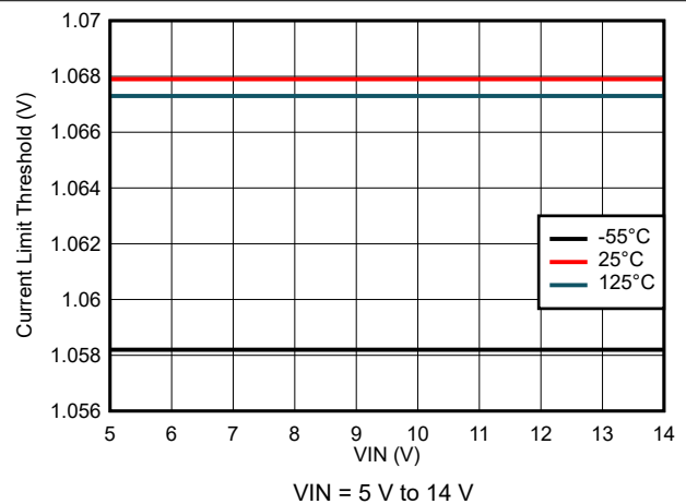
Figure 8-18. Current Limit Threshold Variation
