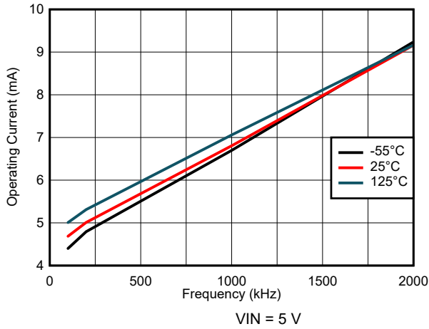
Figure 8-1. Operating Current Variation
