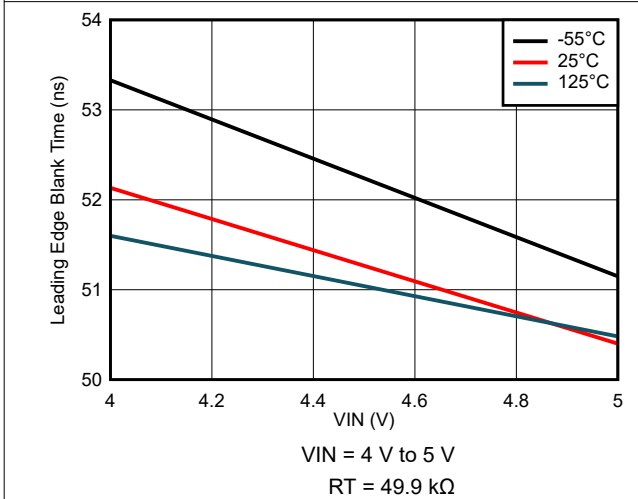
Figure 8-35. Leading Edge Blank Time Variation
