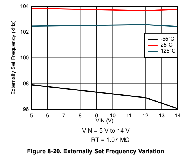
Figure 8-20. Externally Set Frequency Variation
