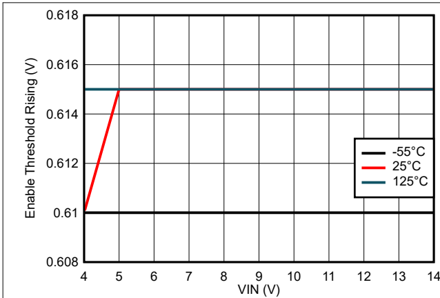
Figure 8-7. Enable Threshold Rising Variation
