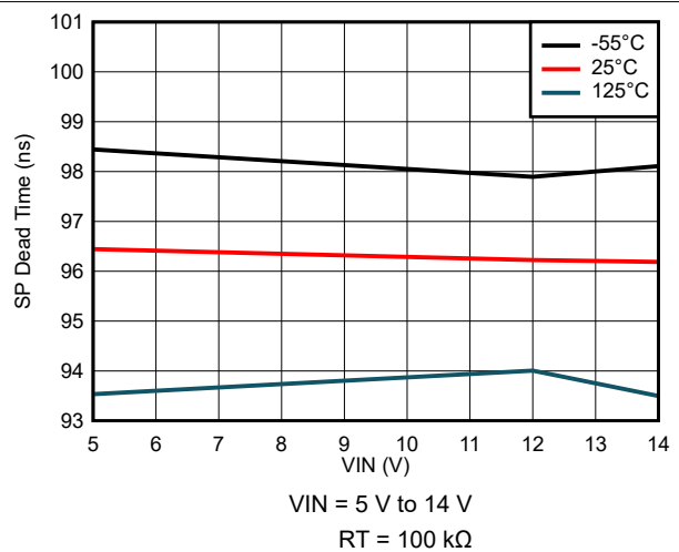
Figure 8-54. SP Dead Time Variation
