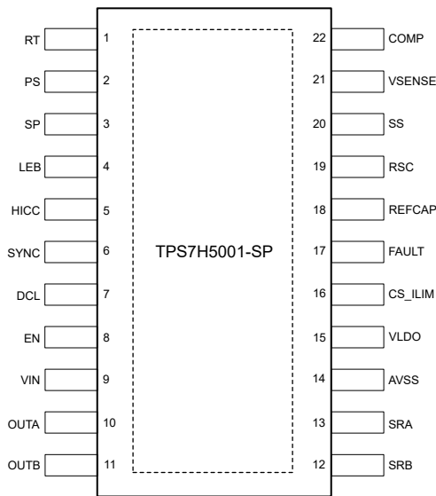
Figure 7-1. TPS7H5001-SP HFT Package 22-Pin CFP With Thermal Pad (Top View)
