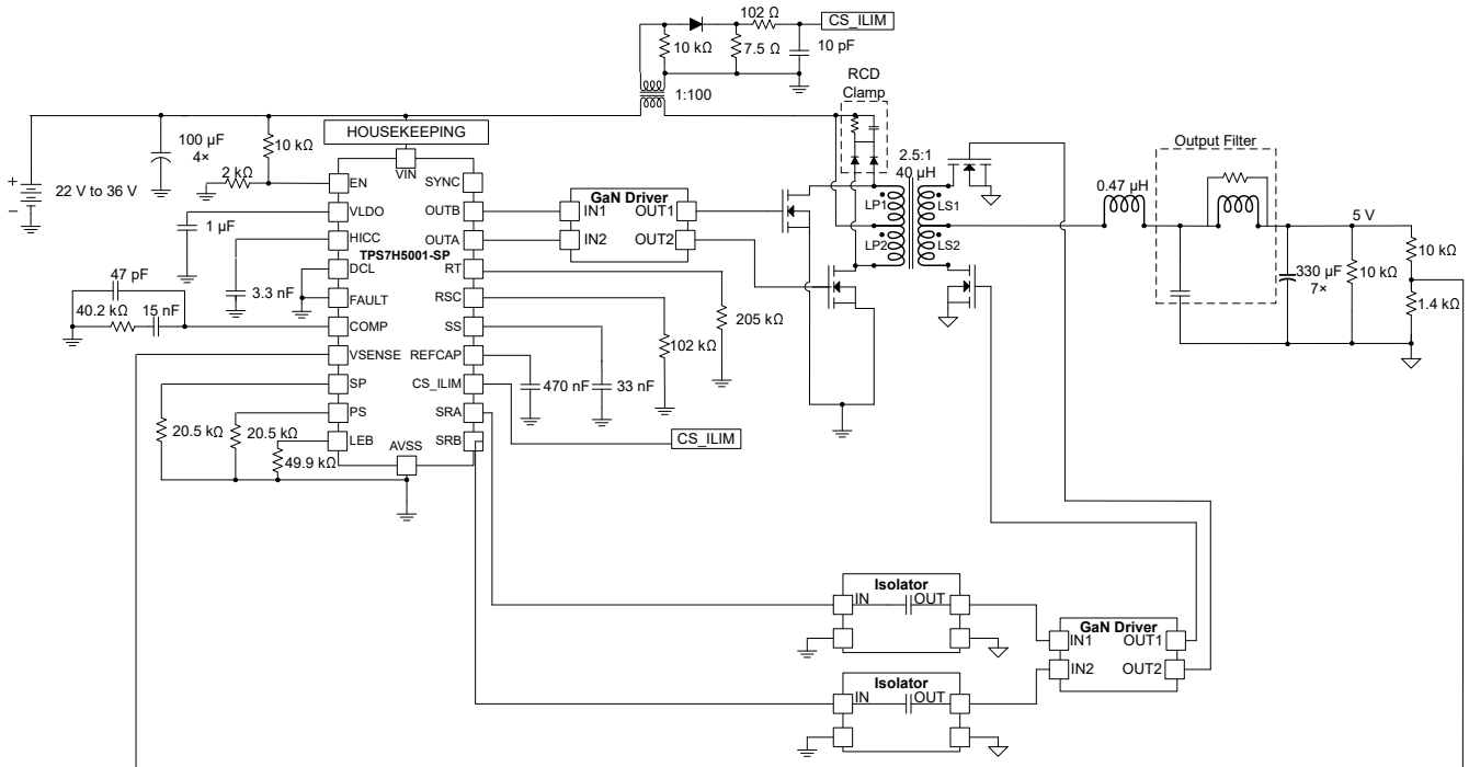
Figure 10-1. Typical Application Schematic
