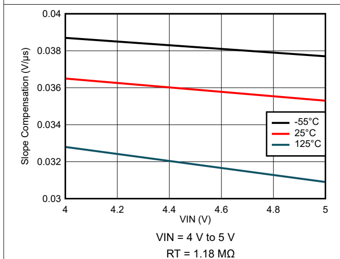
Figure 8-65. Slope Compensation Variation
