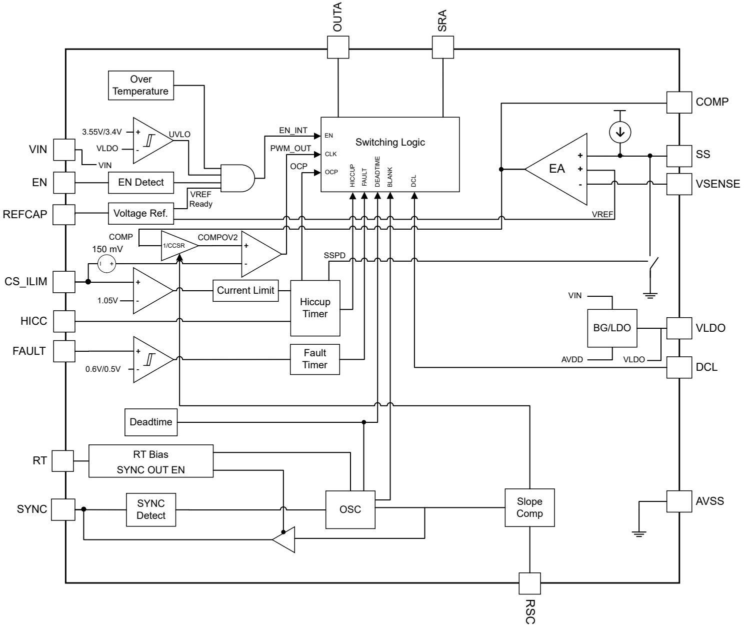
Figure 9-3. TPS7H5003-SP Functional Block Diagram
