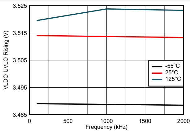
Figure 8-5. VLDO UVLO Rising Variation
