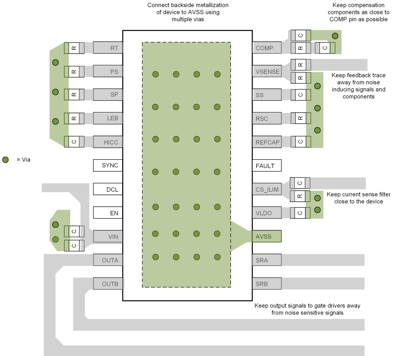
Figure 10-4. PCB Layout Example for CFP Package
