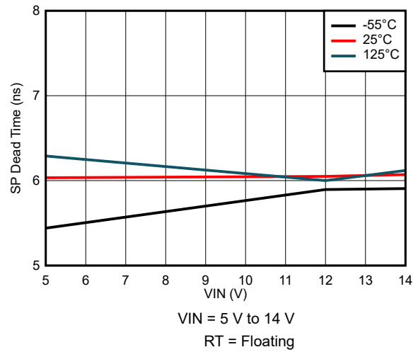
Figure 8-50. SP Dead Time Variation
