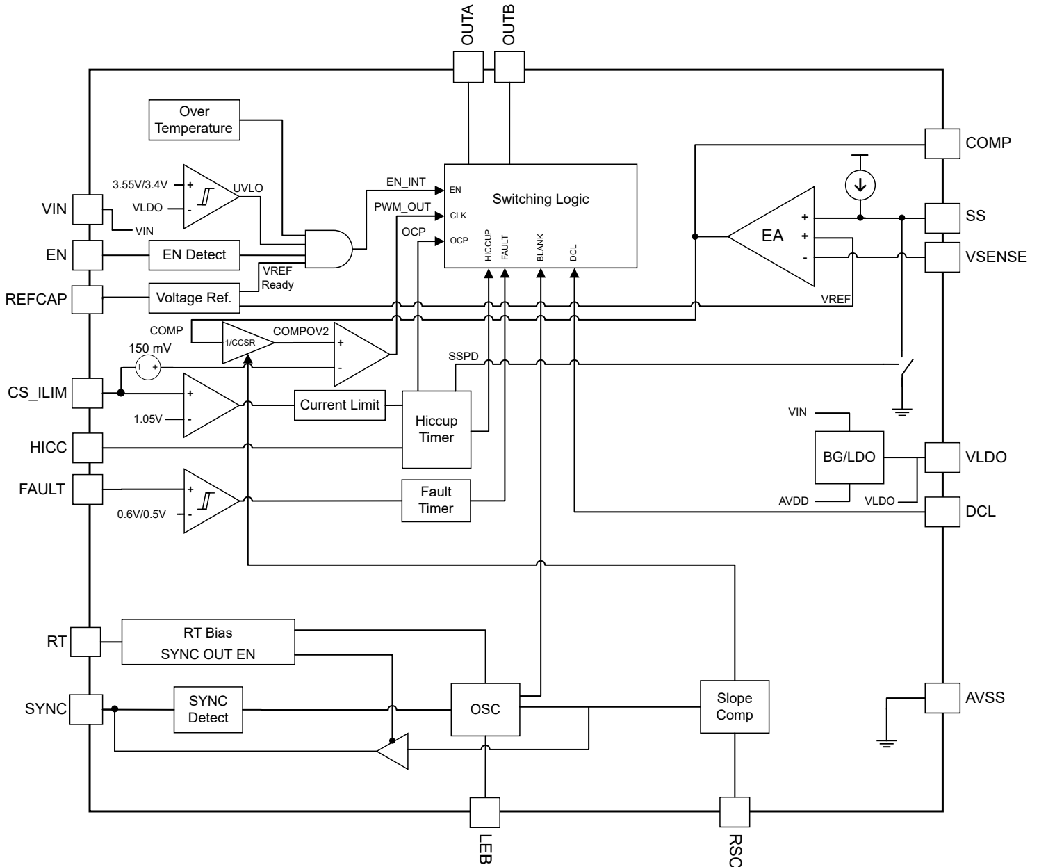
Figure 9-4. TPS7H5004-SP Functional Block Diagram
