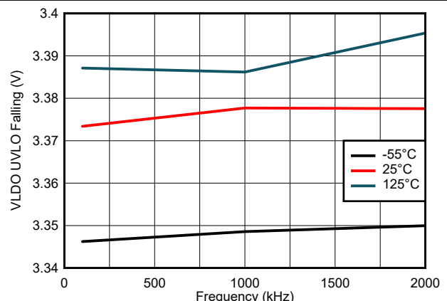
Figure 8-6. VLDO UVLO Falling Variation
