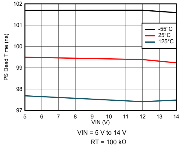
Figure 8-46. PS Dead Time Variation
