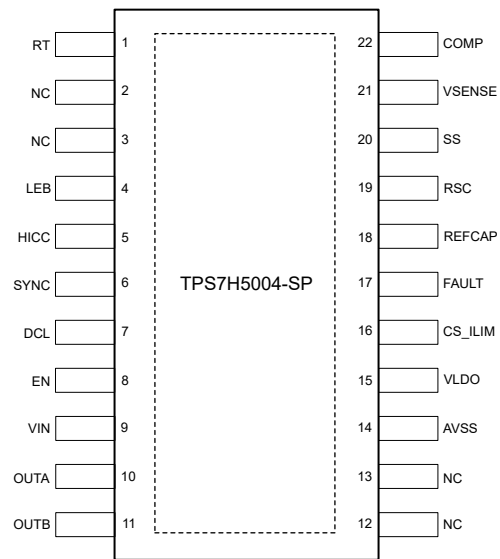
Figure 7-4. TPS7H5004-SP HFT Package 22-Pin CFP With Thermal Pad (Top View)
