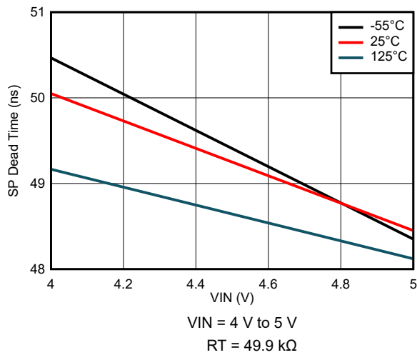
Figure 8-51. SP Dead Time Variation
