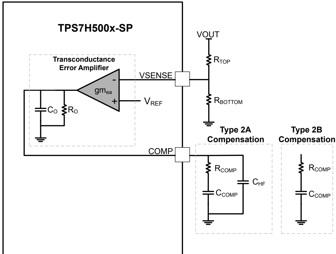
Figure 9-17. TPS7H500x-SP Frequency Compensation Options
