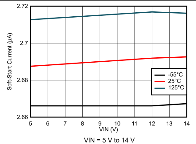
Figure 8-10. Soft-Start Current Variation
