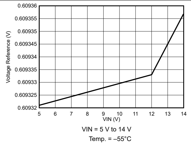
Figure 8-12. Voltage Reference Variation
