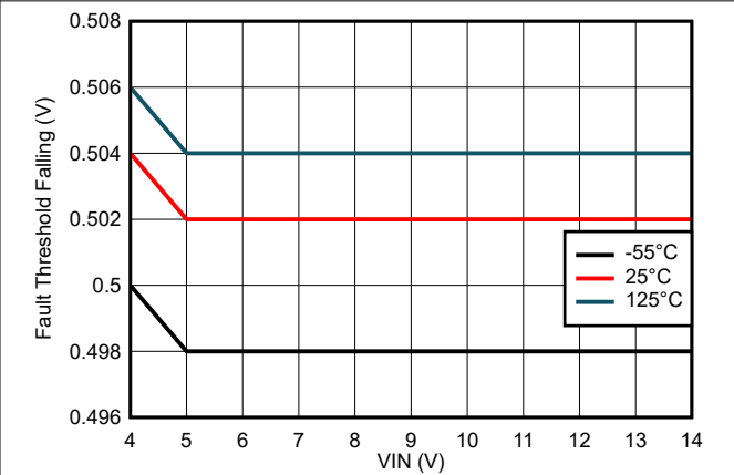
Figure 8-32. FAULT Threshold Falling Variation
