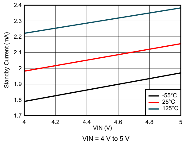
Figure 8-3. Standby Current Variation
