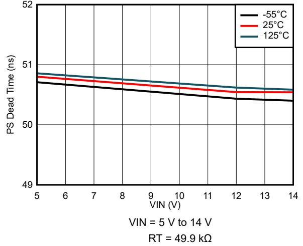
Figure 8-44. PS Dead Time Variation
