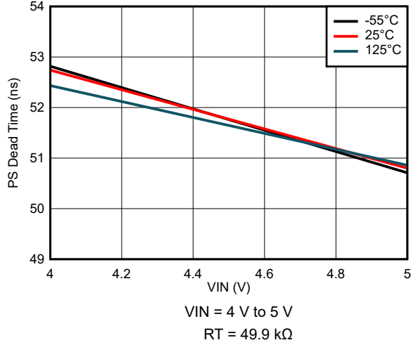
Figure 8-43. PS Dead Time Variation
