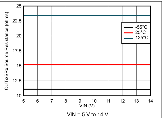
Figure 8-62. Output Source Resistance Variation
