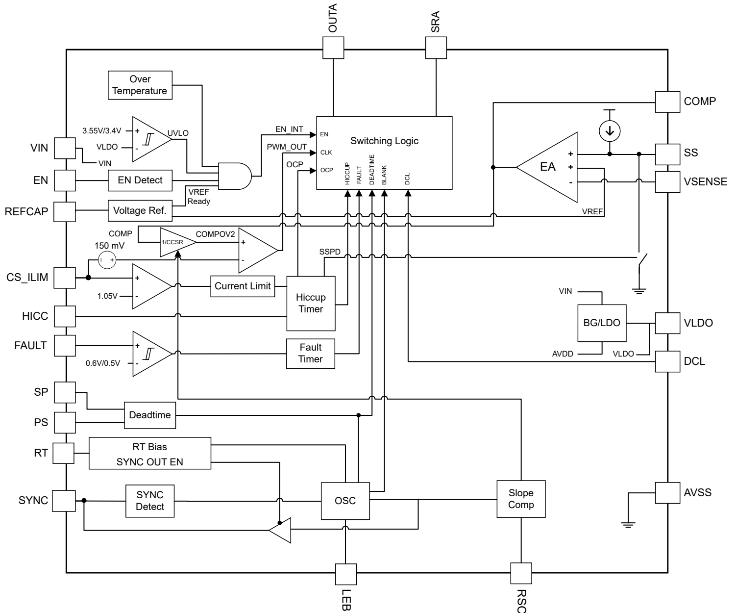
Figure 9-2. TPS7H5002-SP Functional Block Diagram
