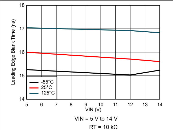
Figure 8-34. Leading Edge Blank Time Variation
