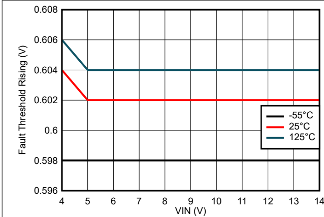
Figure 8-31. FAULT Threshold Rising Variation
