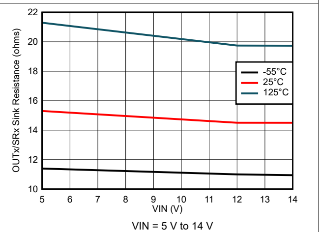
Figure 8-64. Output Sink Resistance Variation
