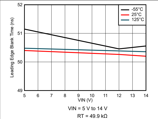
Figure 8-36. Leading Edge Blank Time Variation
