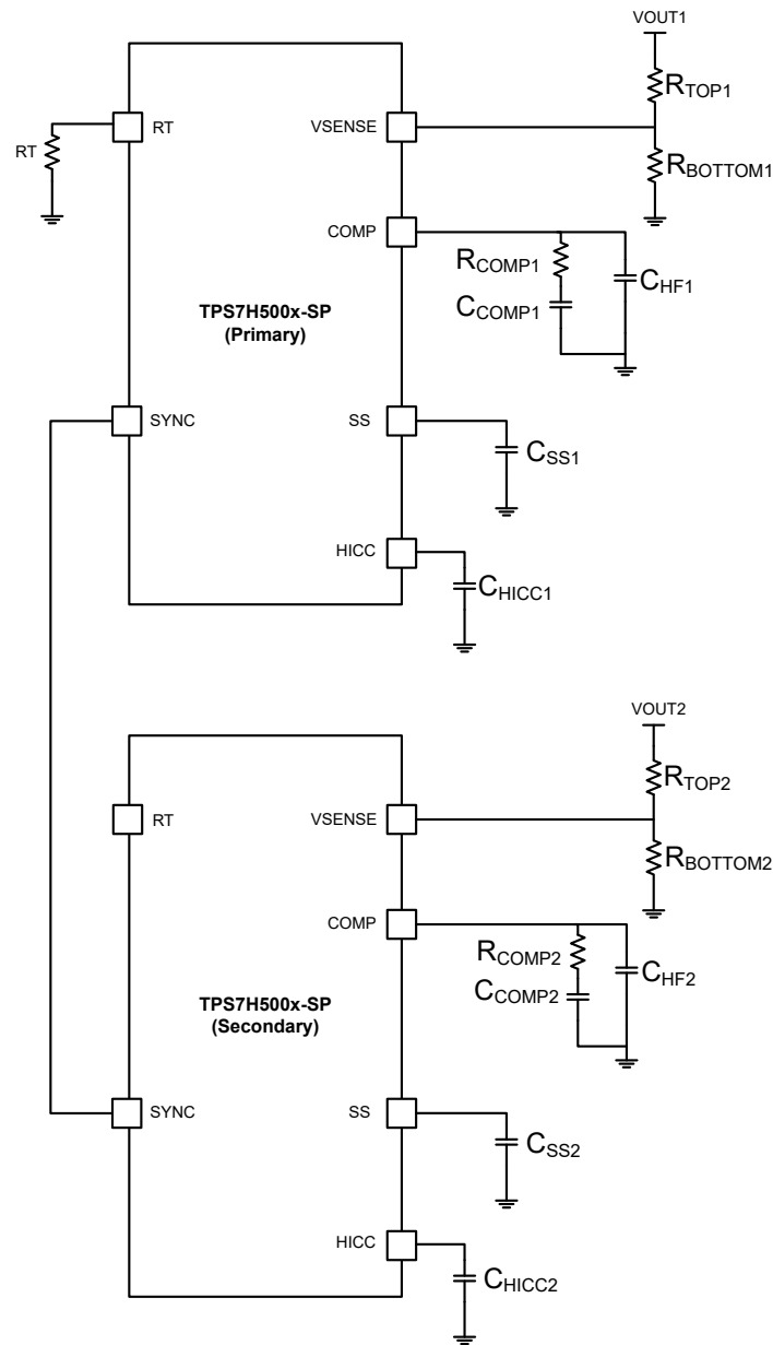
Figure 9-10. Primary-Secondary Mode Configuration for Two Independent Converters
