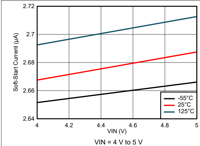
Figure 8-9. Soft-Start Current Variation
