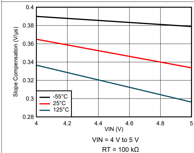
Figure 8-69. Slope Compensation Variation
