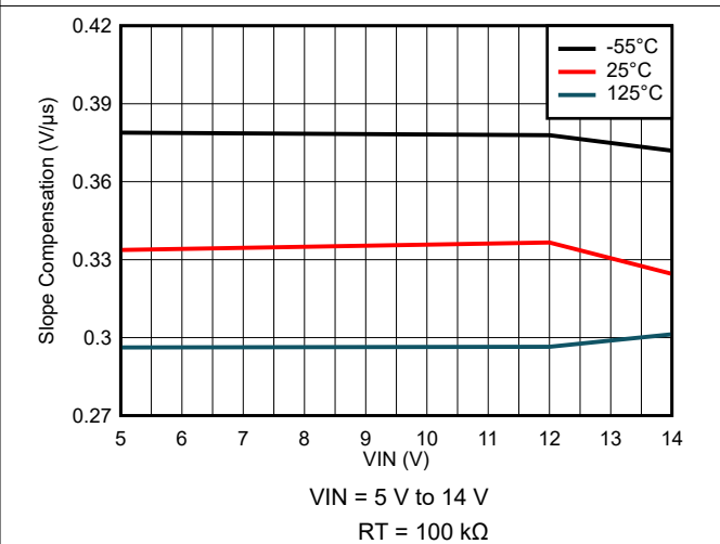
Figure 8-70. Slope Compensation Variation
