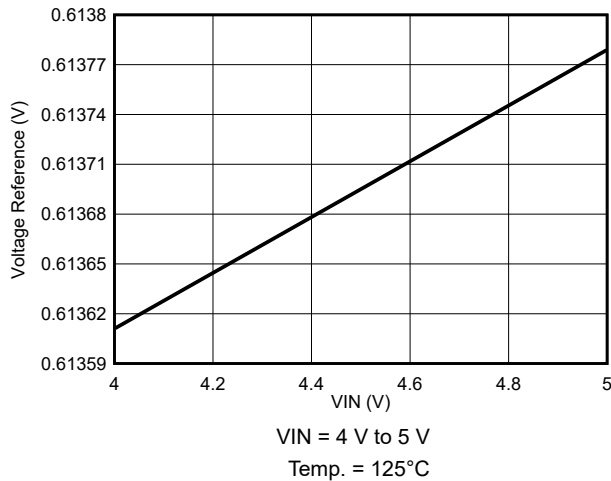
Figure 8-15. Voltage Reference Variation
