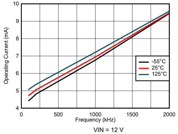
Figure 8-2. Operating Current Variation
