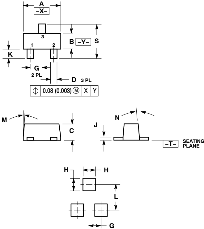
RECOMMENDED PATTERN OF SOLDER PADS
