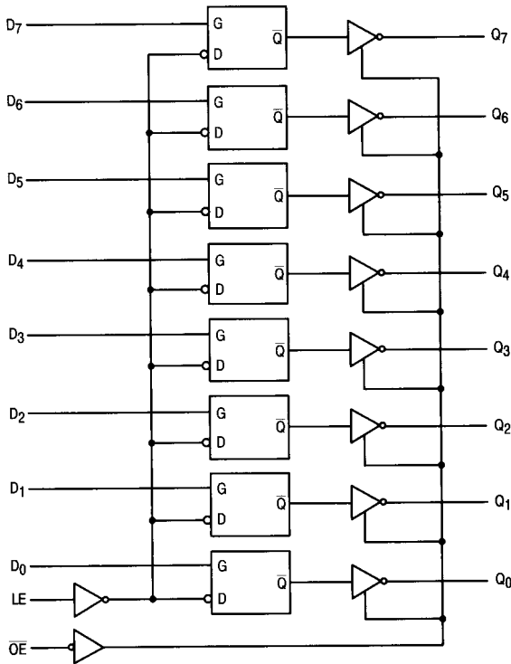
LOGIC DIAGRAM
