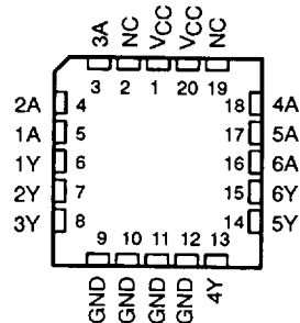
54ACT11034... FK PACKAGE (TOP VIEW)
