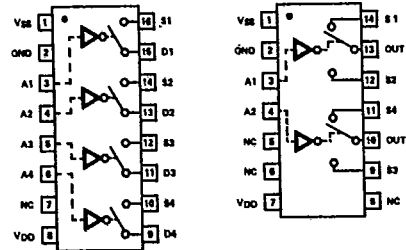
MP7512DI
