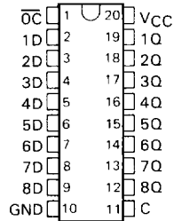
SN54ALS580, SN54AS580 . . . J PACKAGE SN74ALS580, SN74AS580 . . . DW OR N PACKAGE (TOP VIEW)
