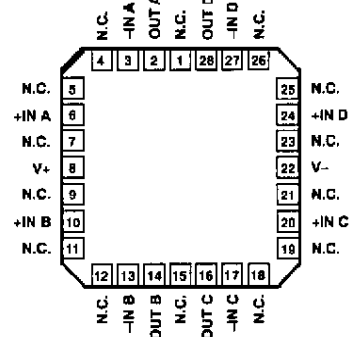
28-LEAD LCC (TC-Suffix)
