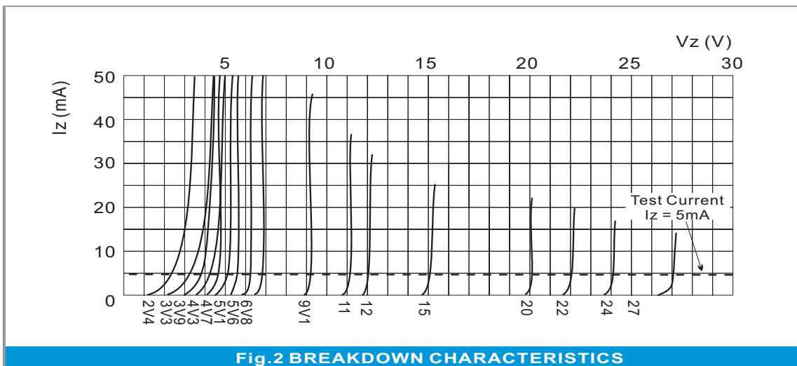
Fig.2 BREAKDOWN CHARACTERISTICS
