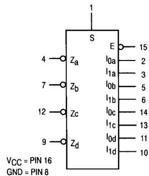
LOGIC SYMBOL
