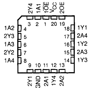
SN54BCT241 ... FK PACKAGE (TOP VIEW)
