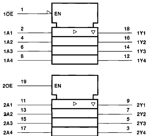
logic symbol†
