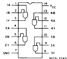
FUNCTIONAL DIAGRAM
