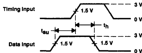
VOLTAGE WAVEFORMS
