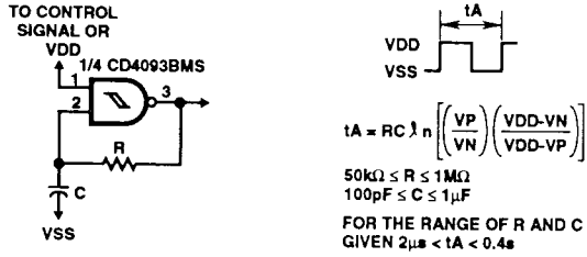
FIGURE 17. ASTABLE MULTIVIBRATOR
