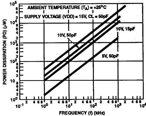
FIGURE 13. TYPICAL POWER DISSIPATION vs. FREQUENCY CHARACTERISTICS
