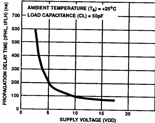
FIGURE 9. TYPICAL PROPAGATION DELAY TIME vs. SUPPLY VOLTAGE
