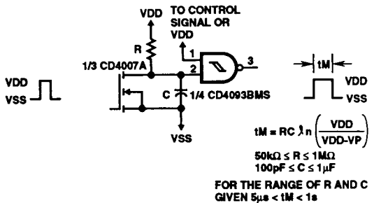
FIGURE 16. MONOSTABLE MULTIVIBRATOR
