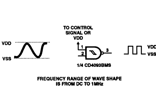
FIGURE 15. WAVE SHAPER
