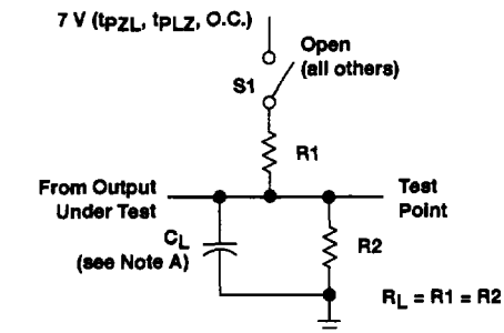
LOAD CIRCUIT FOR 3-STATE AND OPEN-COLLECTOR OUTPUTS
