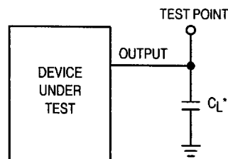
Figure 2. Test Circuit
