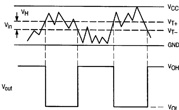
Figure 4. Typical Schmitt-Trigger Applications
