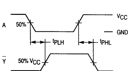
Figure 1. Switching Waveforms
