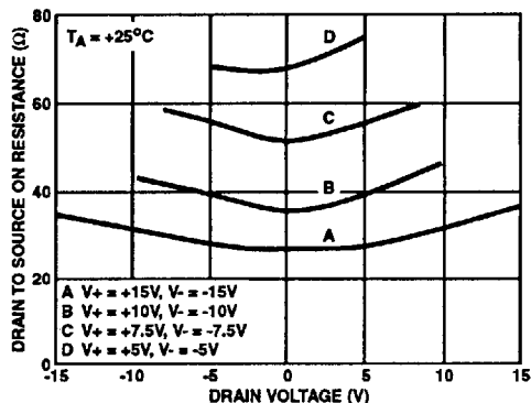
FIGURE 2. R_{DS(ON)} vs V_D AND POWER SUPPLY VOLTAGE
