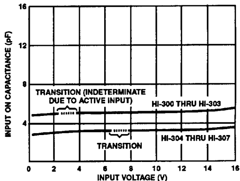
FIGURE 9. DIGITAL INPUT CAPACITANCE vs INPUT VOLTAGE
