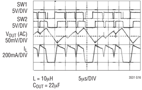
4 Switch Mode Waveforms at 3.6V_{IN} , 3.3V_{OUT} 200mA
