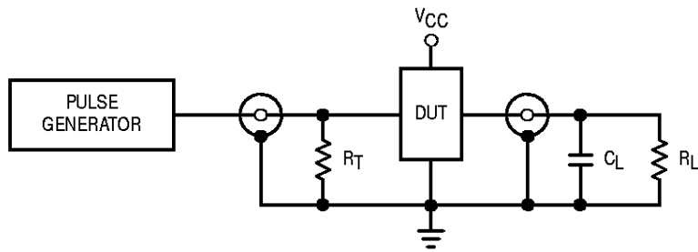
C_L = 50pF or equivalent (Includes jig and probe capacitance) R_L = R_1 = 500\Omega or equivalent R_T = Z_{OUT} of pulse generator (typically 50\Omega )
