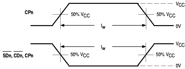
WAVEFORM 4 – PULSE WIDTH t_R = t_F = 2.5ns (or fast as required) from 10% to 90%; Output requirements: V_{OL} \leq 0.8V, V_{OH} \geq 2.0V
