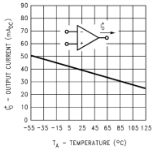
Current Limiting
