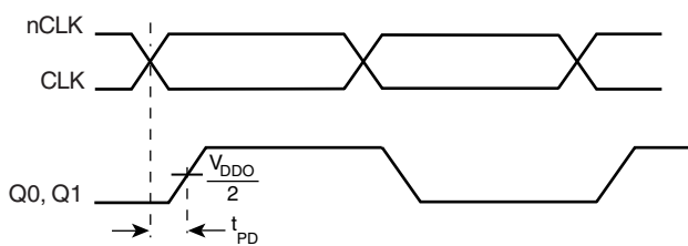
PROPAGATION DELAY
