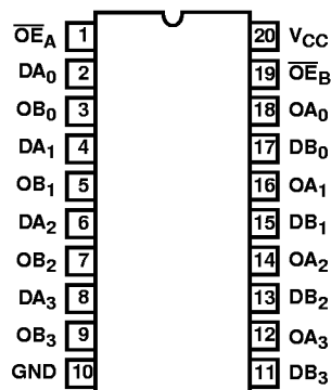
CD74LPT244 (SOIC, QSOP) TOP VIEW
